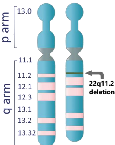
Chromosome 22
